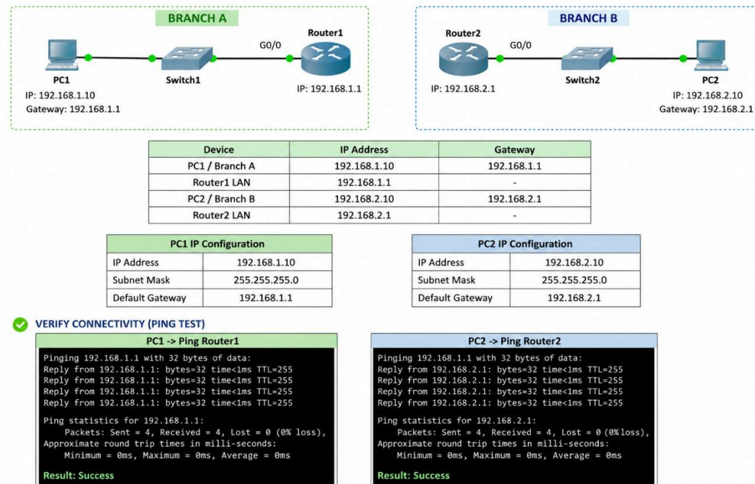
Figure 1: Basic site-to-site VPN topology
